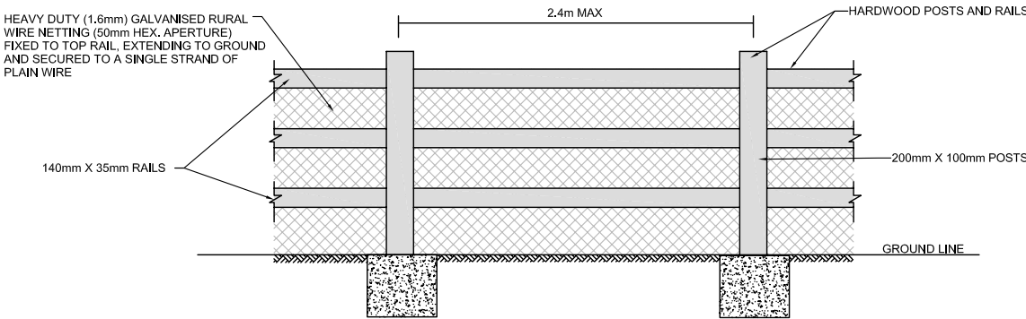
HERITAGE FENCE DETAIL 1:25
