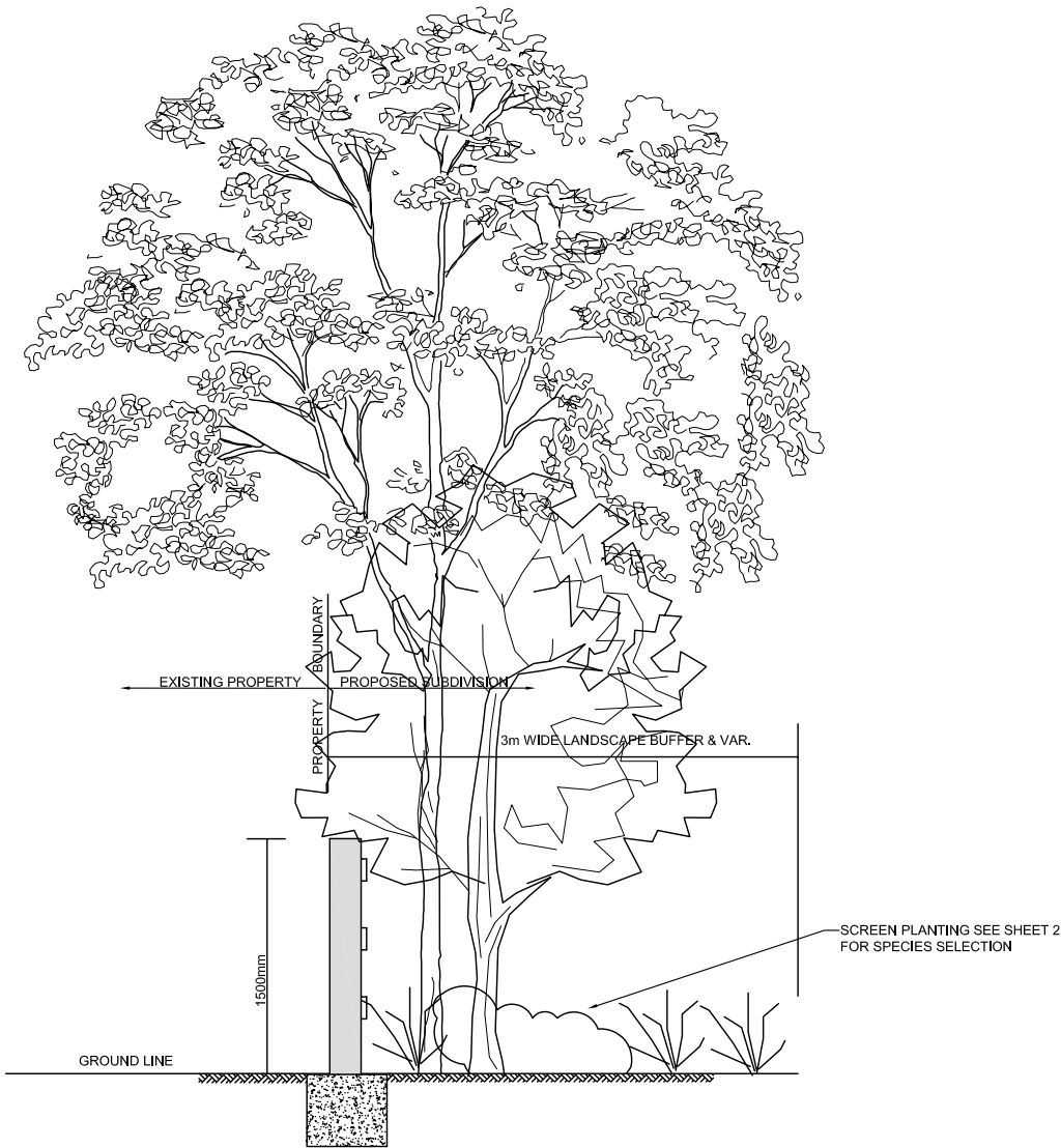
HERITAGE FENCE & PLANTED SCREEN DETAIL 1:25
